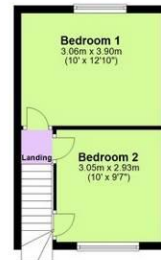
First Floor Approx. 24.2 sq. metres (260.6 sq. feet)
