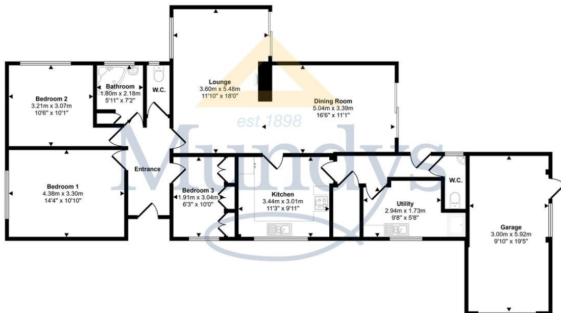
Floorplan
