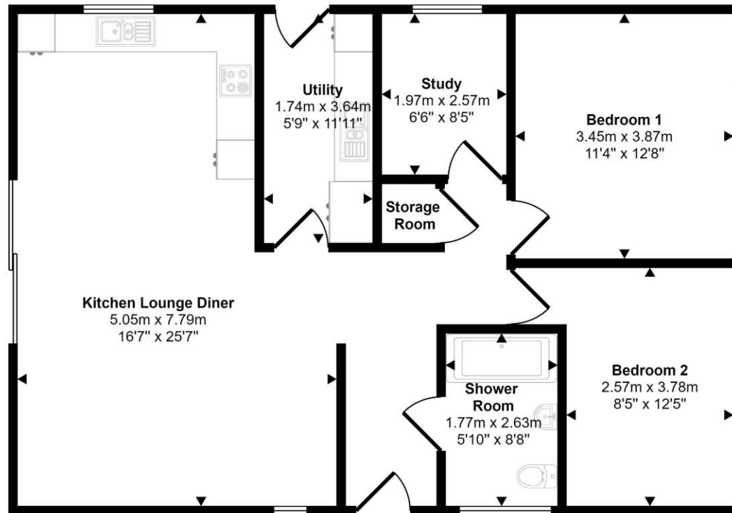
Floorplan
