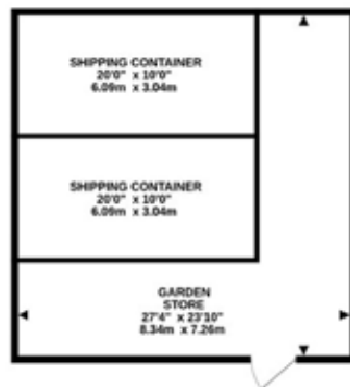
OUTBUILDINGS 1464 sq.ft. (136.0 sq.m.) approx.
