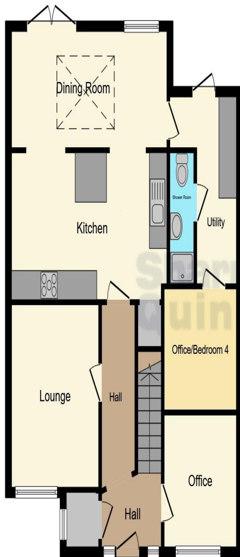
Ground Floor
