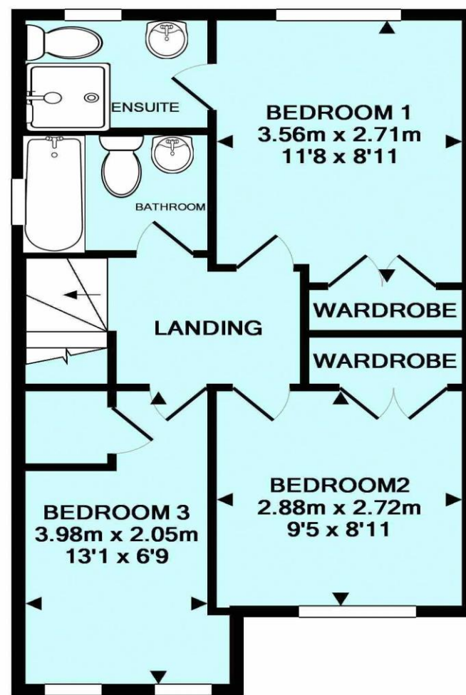
1ST FLOOR APPROX. FLOOR AREA 39.5 SQ.M. (425 SQ.FT.)
