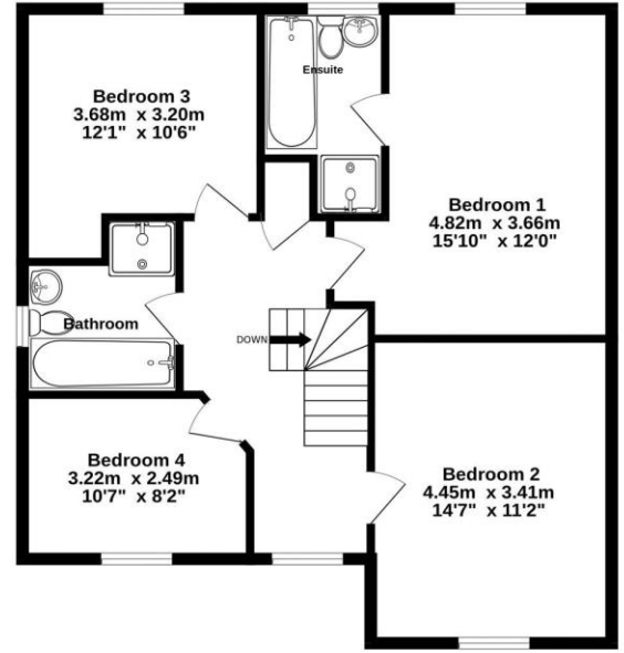
1st Floor 71.6 sq.m. (771 sq.ft.) approx.
