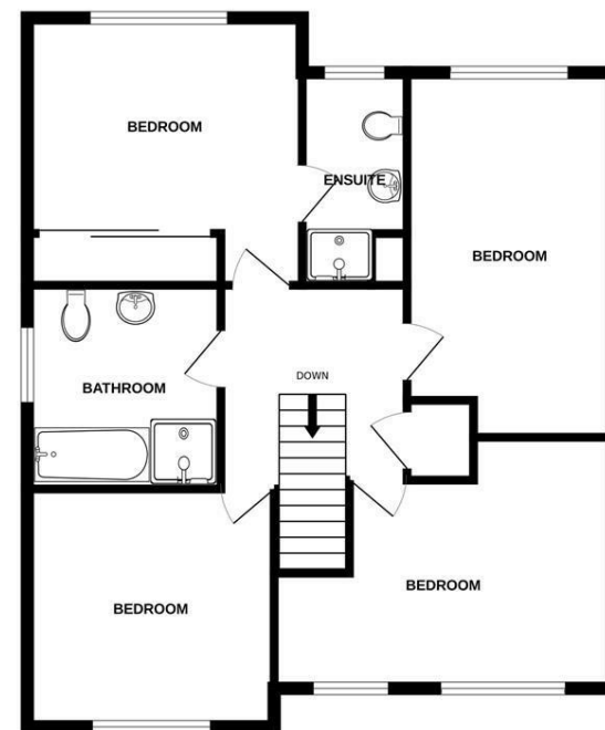
1ST FLOOR 755 sq.ft. (70.1 sq.m.) approx.
