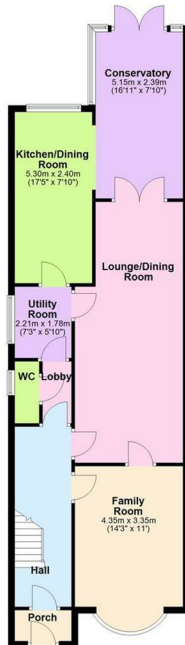
Ground Floor
