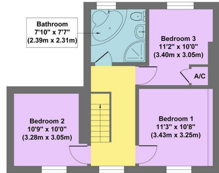
First Floor Approximate Floor Area 473 sq.ft (43.94 sq.m.)
