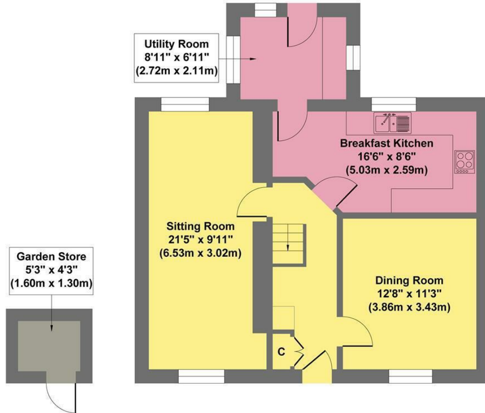
Outbuilding Approximate Floor Area 22 sq.ft (2.04 sq.m.)
