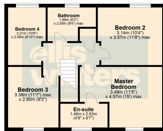
First Floor Approx. 57.4 sq. metres (618.2 sq. feet)
