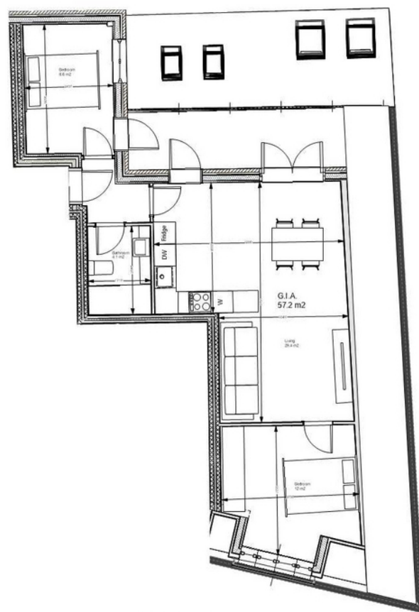
1 Flat L - Second floor Scale 1:50
