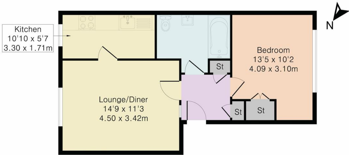
Second Floor Flat
