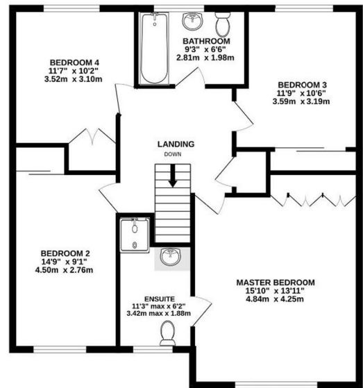
1ST FLOOR 867 sq.ft. (80.5 sq.m.) approx.
