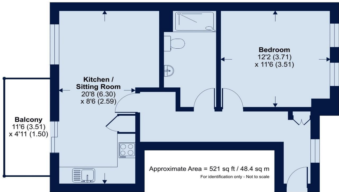
FIRST FLOOR
