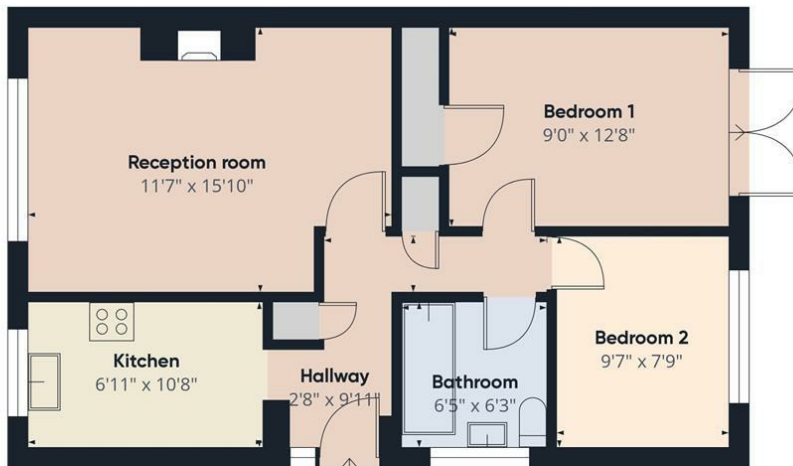
Floor 0 Building 1
