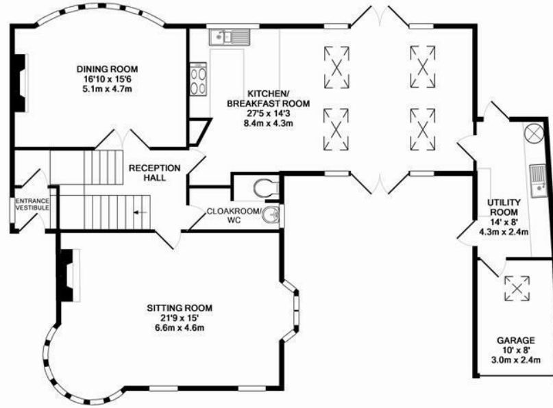
GROUND FLOOR APPROX. FLOOR AREA 1318 SQ.FT. (122.5 SQ.M.)
