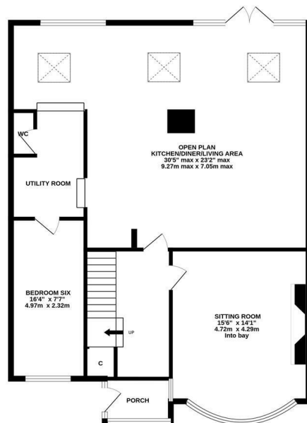
GROUND FLOOR 1161 sq.ft. (107.9 sq.m.) approx.
