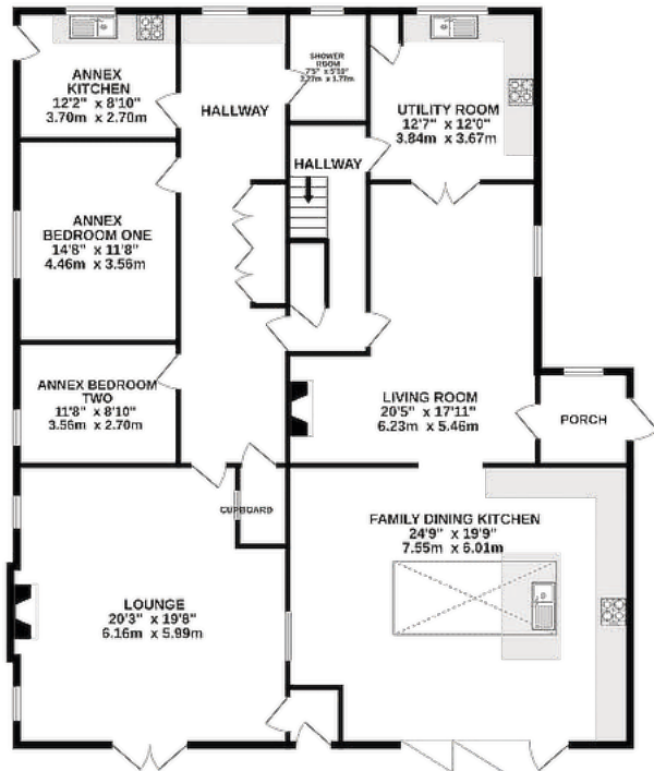
GROUND FLOOR 2250 sq.ft. (209.0 sq.m.) approx.
