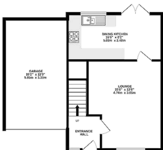
GROUND FLOOR 601 sq.ft. (55.8 sq.m.) approx.
