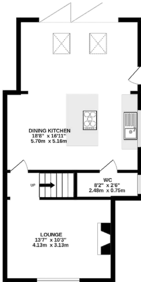
GROUND FLOOR 494 sq.ft. (45.9 sq.m.) approx.
