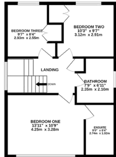
1ST FLOOR 508 sq.ft. (47.2 sq.m.) approx.
