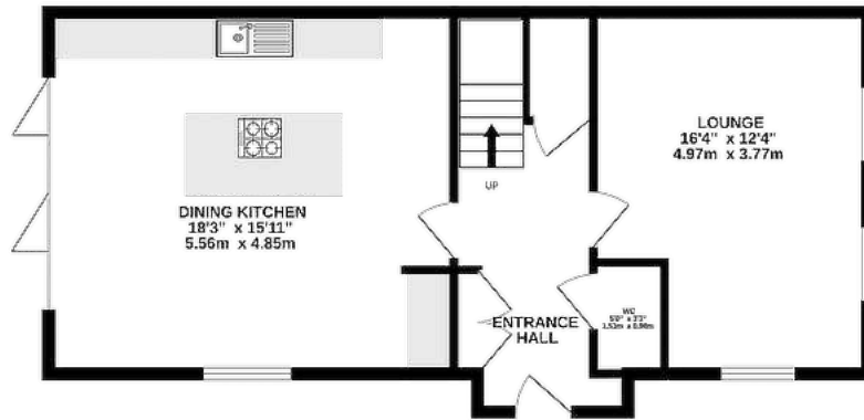
GROUND FLOOR 612 sq.ft. (56.9 sq.m.) approx.
