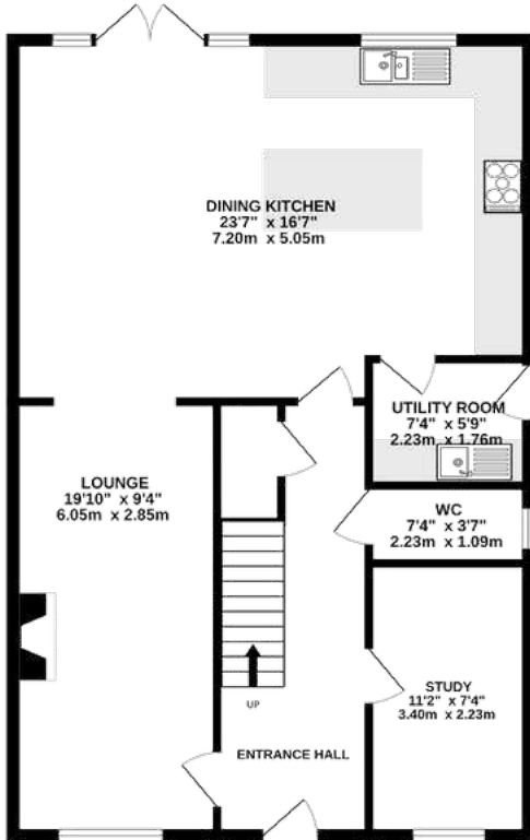
GROUND FLOOR 853 sq.ft. (79.3 sq.m.) approx.
