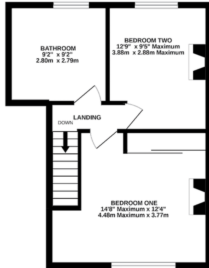
1ST FLOOR 376 sq.ft. (34.9 sq.m.) approx.
