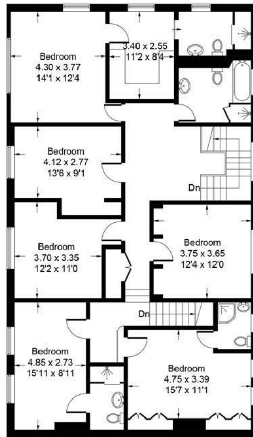
First Floor = 1579 sq ft / 146.7 sq m
