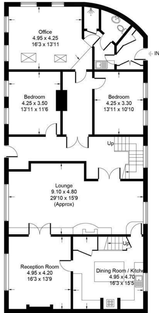
Ground Floor = 1976 sq ft / 183.6 sq m
