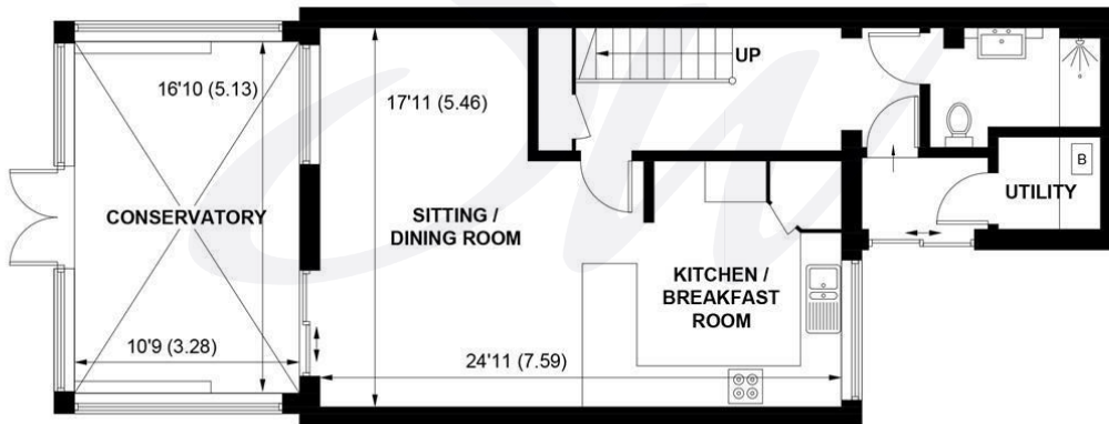
GROUND FLOOR
