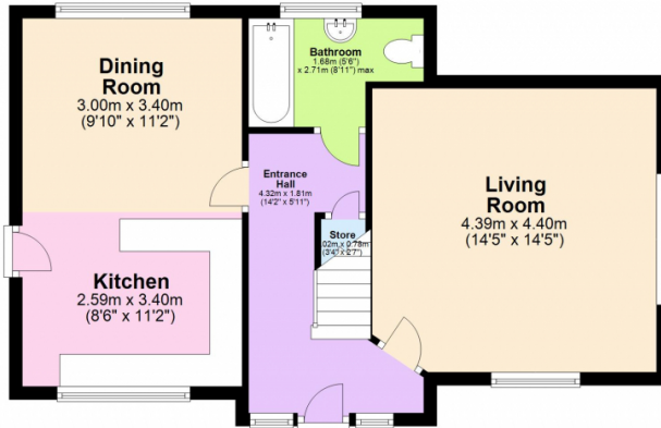
Ground Floor Approx. 52.3 sq. metres (563.4 sq. feet)
