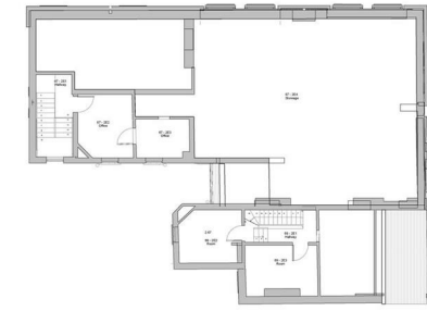
1) Level 2 - Existing
