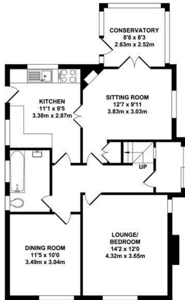
GROUND FLOOR APPROX. FLOOR AREA 804 SQ.FT. (74.71 SQ.M.)
