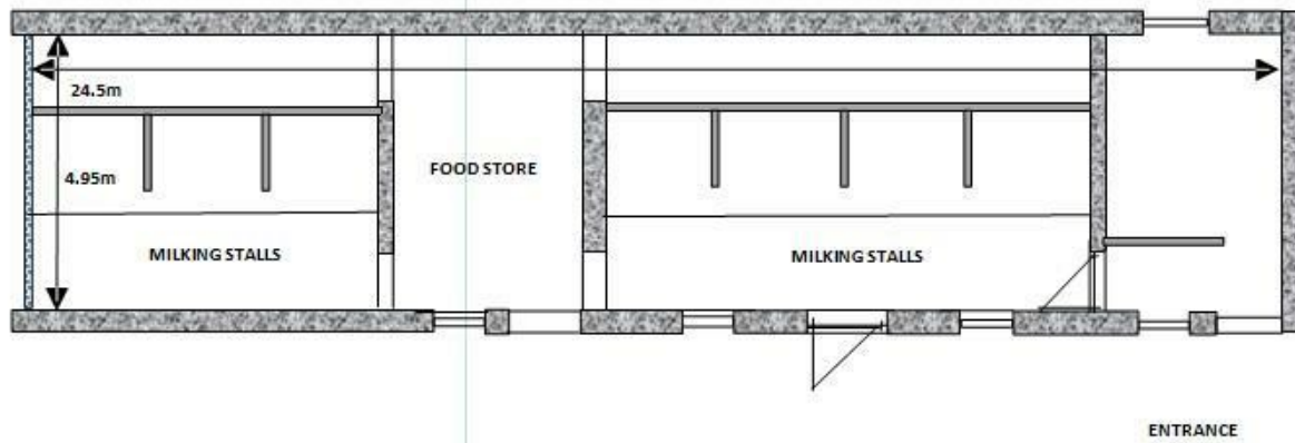
Plan 6
