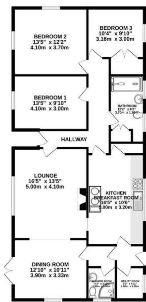
GROUND FLOOR 1230 sq.ft. (114.3 sq.m.) approx.
