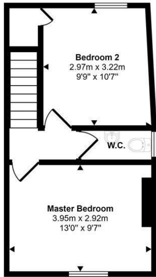
First Floor Approx 28 sq m / 303 sq ft
