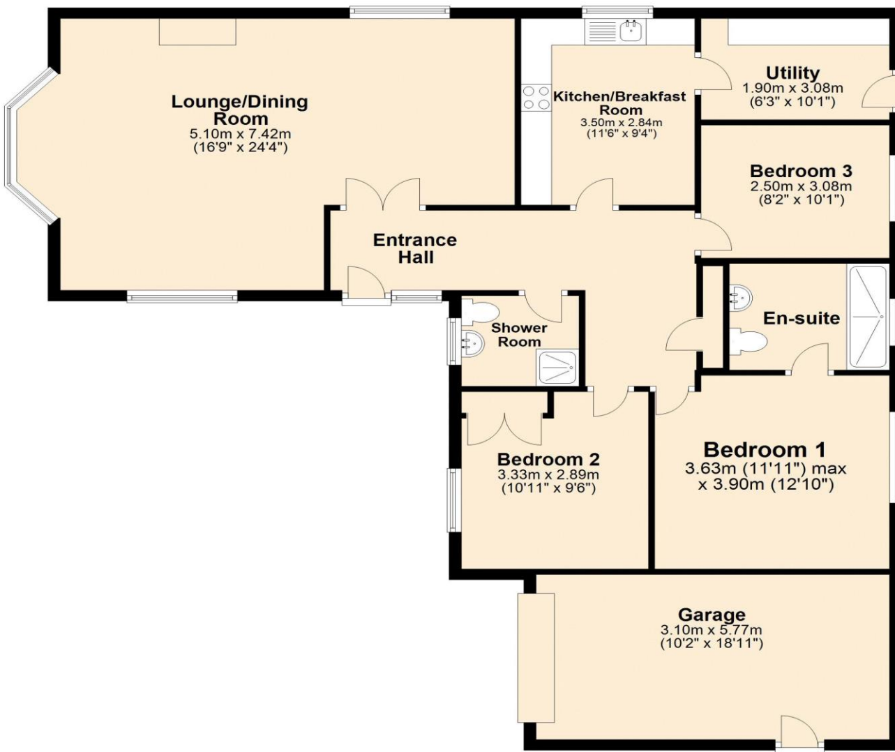
Ground Floor Approx. 123.7 sq. metres (1331.1 sq. feet)
