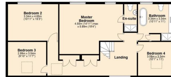
First Floor Approx. 99.7 sq. metres (1072.8 sq. feet)
