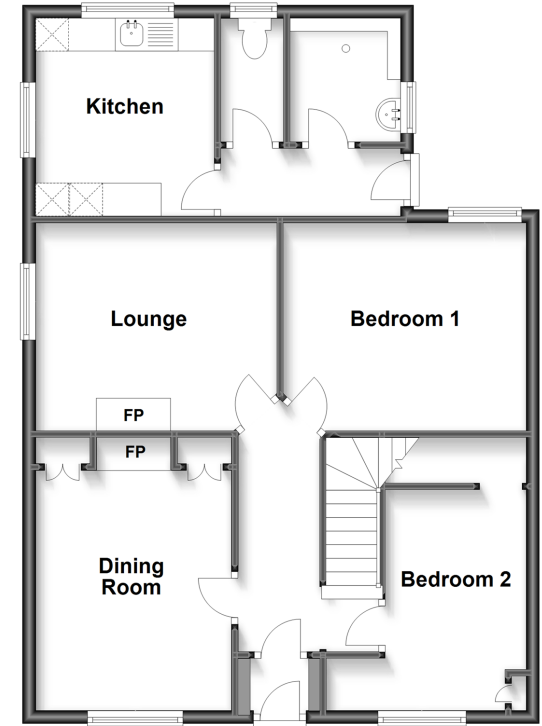
Ground Floor Approx. 72.6 sq. metres (781.5 sq. feet)
