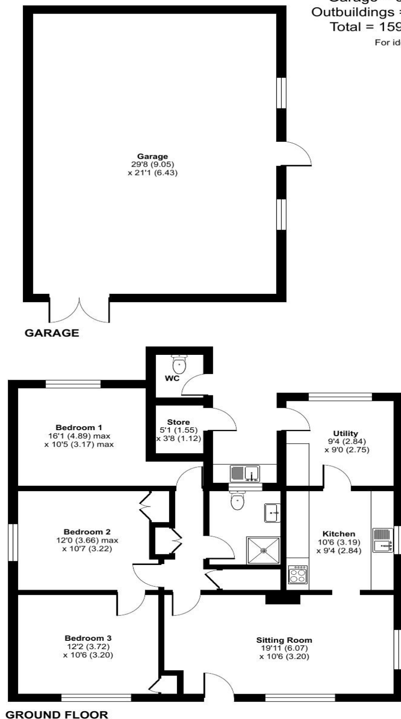
GROUND FLOOR
