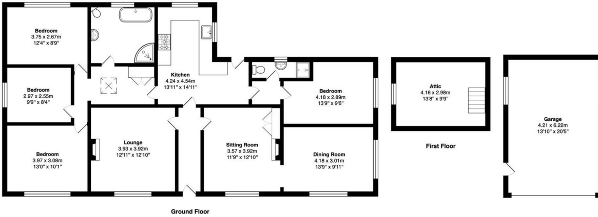
Ground Floor
