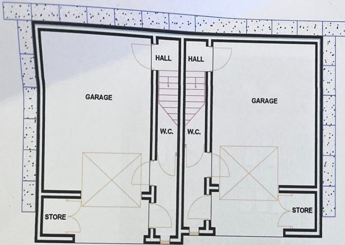
PROPOSED LOWER GROUND FLOOR PLAN
