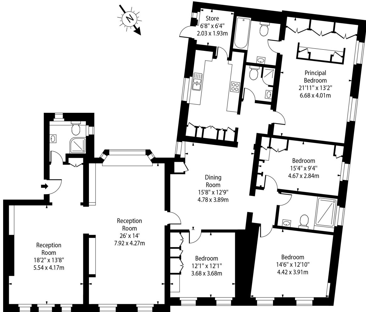
Third Floor
