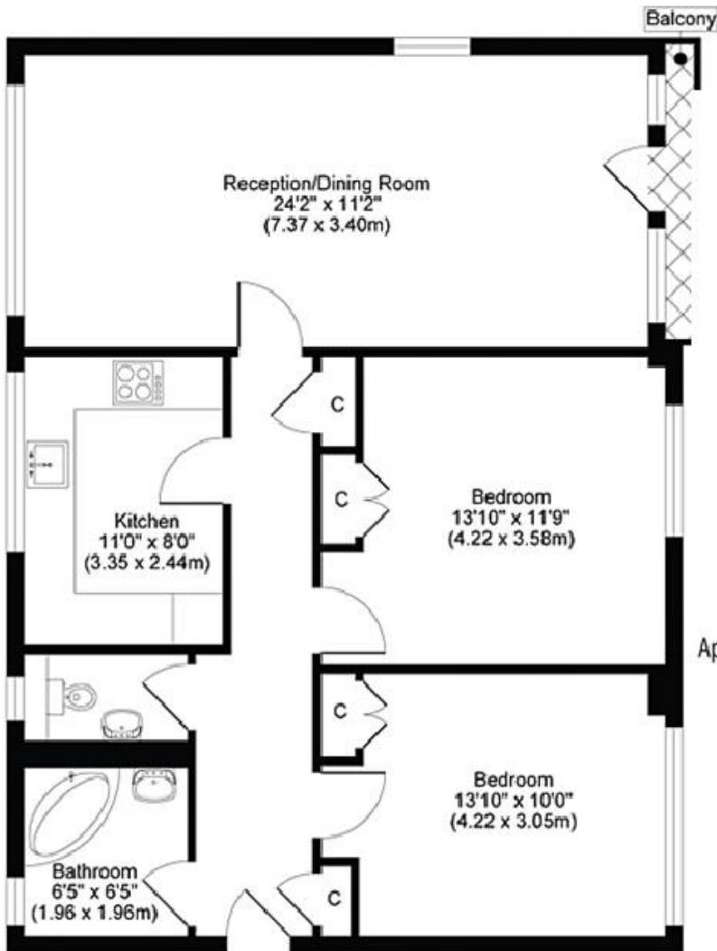
GROUND FLOOR
