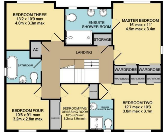
FIRST FLOOR APPROX. FLOOR AREA 981 SQ.FT. (91.1 SQ.M.)
