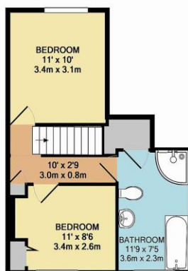
1ST FLOOR APPROX. FLOOR AREA 361 SQ.FT. (33.6 SQ.M.)
