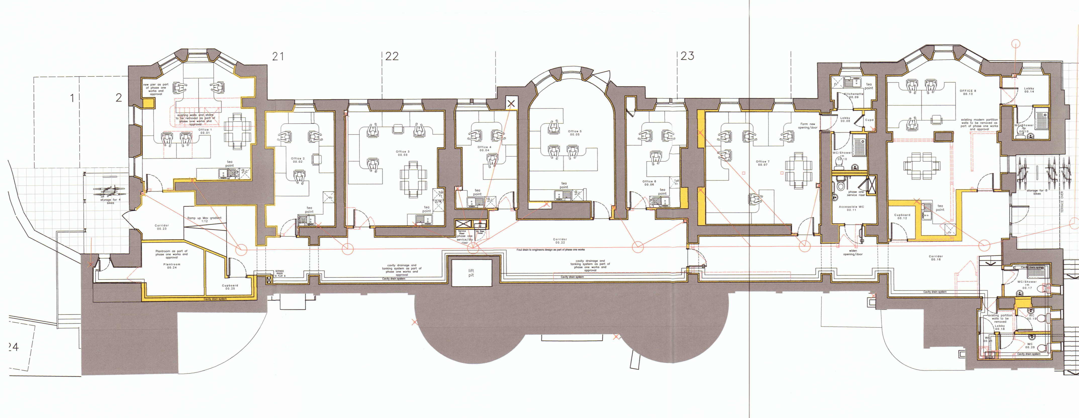
Basement Plan as Proposed
