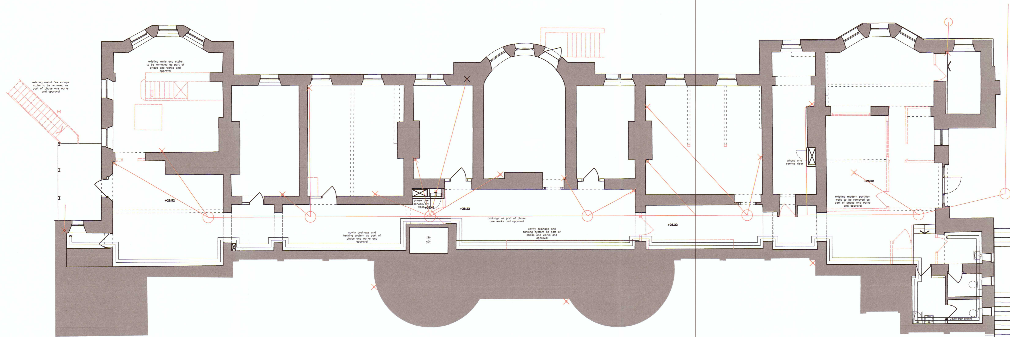
Basement Plan as Existing
