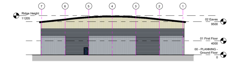
PLANNING - Rear Elevation 1 : 200
