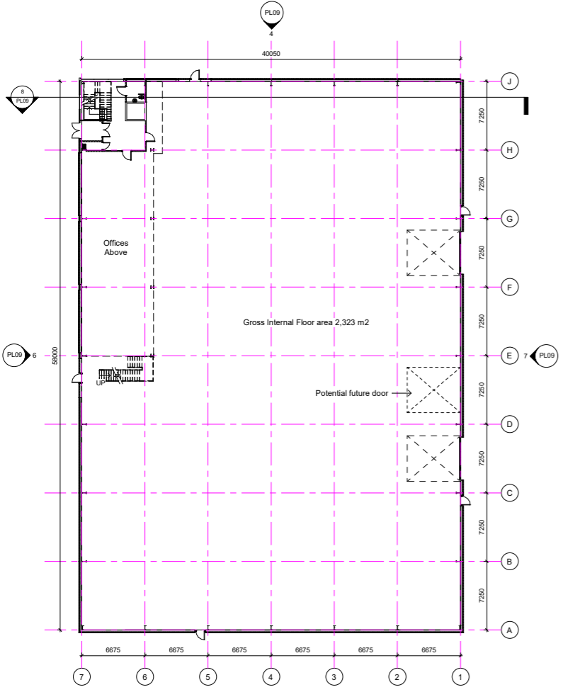
00 - PLANNING - Ground Floor 1 : 200
