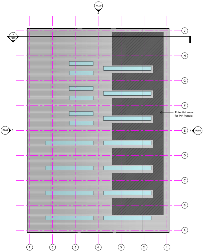
02 - PLANNING - Roof Plan 1 : 200
