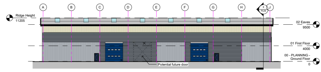
PLANNING - Side Elevation (2) 1 : 200
