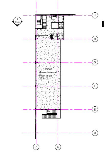
01 - PLANNING - First Floor 1 : 200
