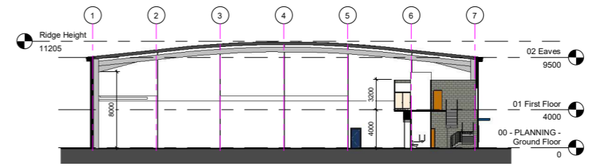
PLANNING - Section 1 1 : 200
