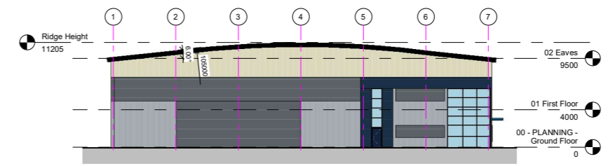
PLANNING - Front Elevation 1 : 200
