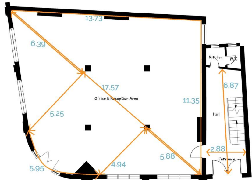
Ground Floor Plan 1,837 sq.ft (170.67 sq.m)
