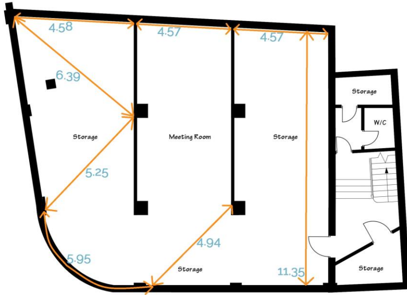
Basement Plan 1,837 sq.ft (170.67 sq.m)
