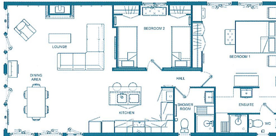
45' x 22' two bedrooms, en-suite and shower-room
