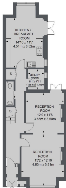
GROUND FLOOR
