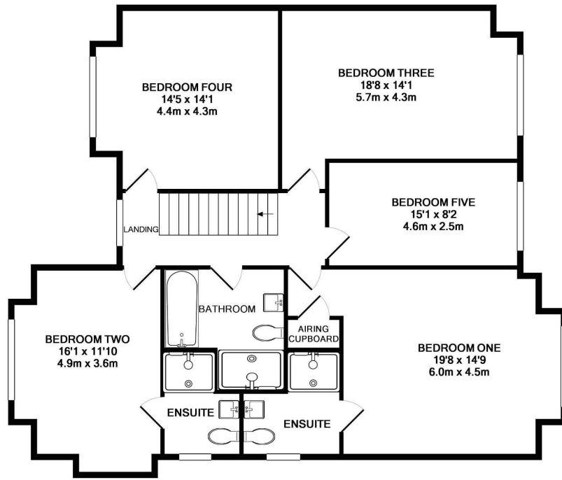
1ST FLOOR APPROX. FLOOR AREA 1273 SQ.FT. (118.3 SQ.M.)
